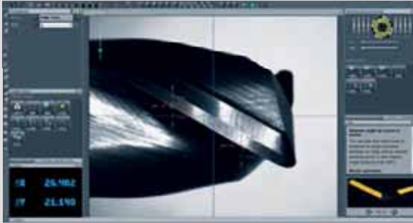
Determination of chamfer width and spiral angle.
