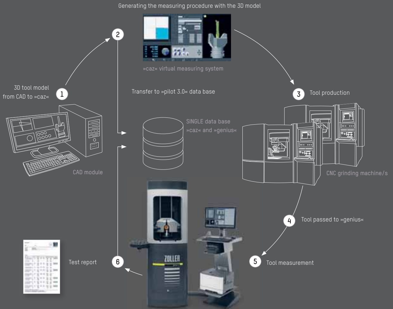
ZOLLER »genius« | Automatic measurement of tools
